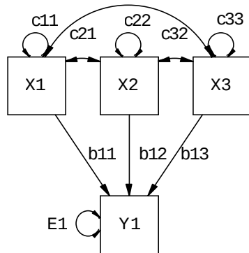
d) multivariate regression (case 2)
