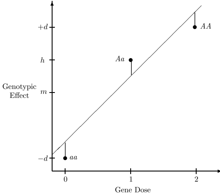
Figure 3.2: Regression of genotypic effects on gene dosage showing additive and dominance effects under random mating. The figure is drawn to scale for u = v = \frac{1}{2} , d = 1 , and h = \frac{1}{2} .
