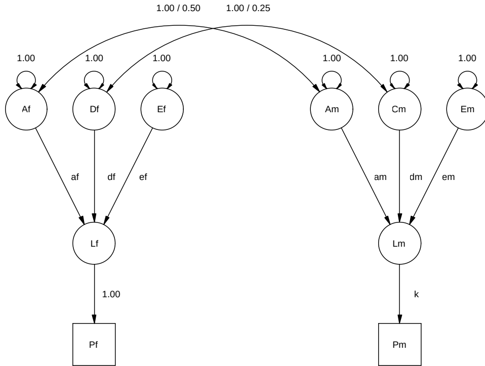
Figure 9.2: The scalar genotype \times sex interaction model for twin data. Path diagram is shown for DZ opposite-sex twin pairs. The \alpha = 0.5 and \beta = 0.25 .
