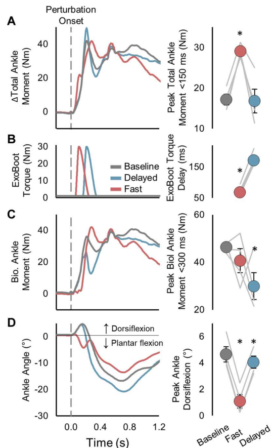
Fig. 4. Ankle mechanics. Left: Time series data of average (A) net ankle moment, (B) ExoBoot torque, (C) net biological (Biol) ankle moments, and (D) ankle angle. Right: Average \pm SE (A) peak ankle moment within 150 ms after perturbation magnitude, (B) delay between perturbation onset and ExoBoot torque onset, (C) peak biological ankle moment production throughout the support surface translation (0 to 500 ms), and (D) peak change in ankle dorsiflexion throughout the support surface translation, with individual participant data (gray). Panels contain n = 4 , except for (B), which includes n = 8 . We only displayed participants who performed successful, balance-maintained trials in each ExoBoot condition at the same perturbation magnitude. Statistics pertain to all analyzed participants across multiple perturbation magnitudes ( n = 9 ). Asterisks (*) denote significance between the indicated artificially fast or physiologically delayed ExoBoot condition and baseline ( P < 0.05 ).
